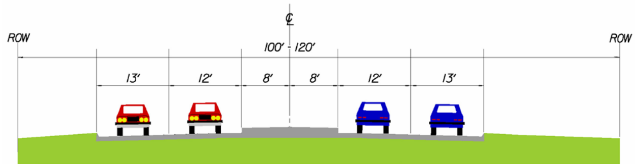
4-Lane Divided Arterial
